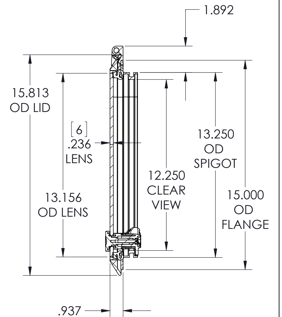
SECTION B-B
